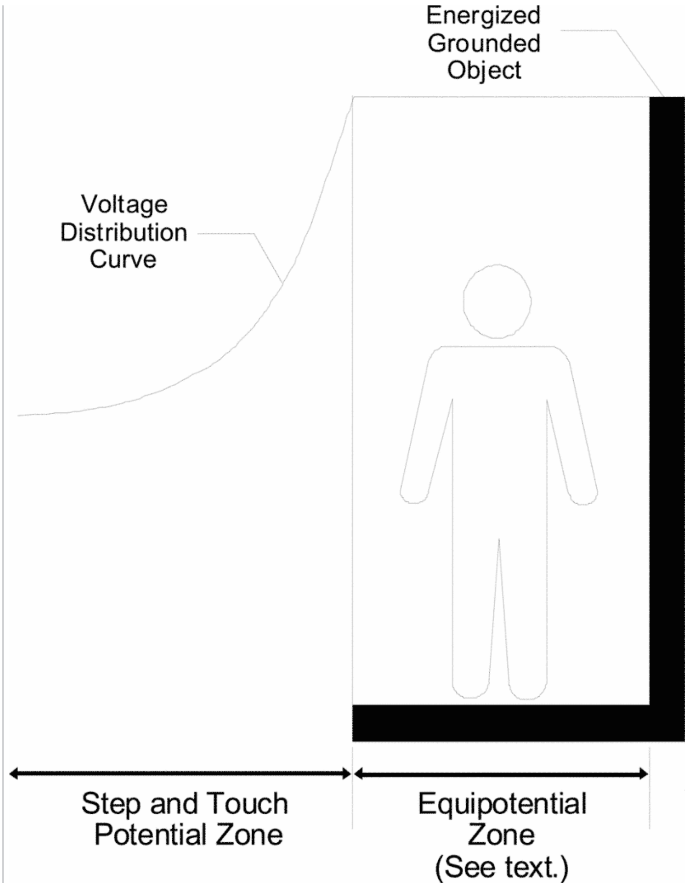
Figure 3—Protection from Ground-Potential Gradients
