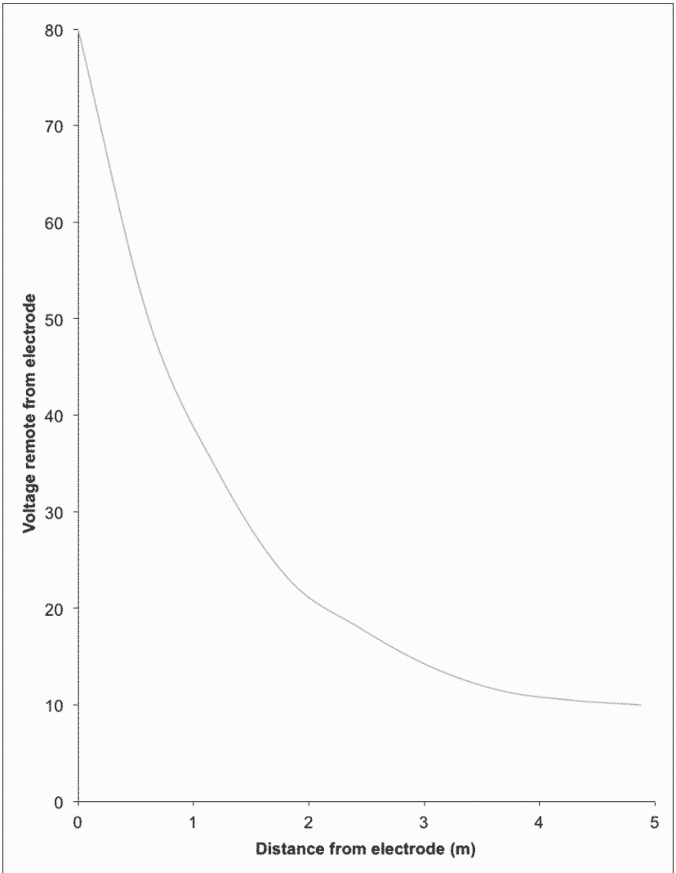
Figure 1—Typical Voltage-Gradient Distribution Curve
