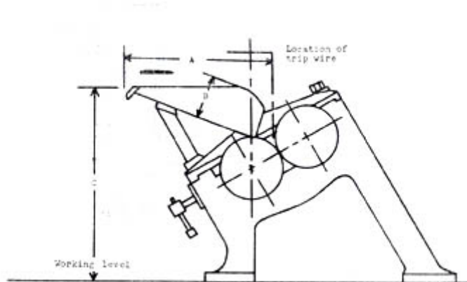
Section through centre line of oblique set of rolls.
